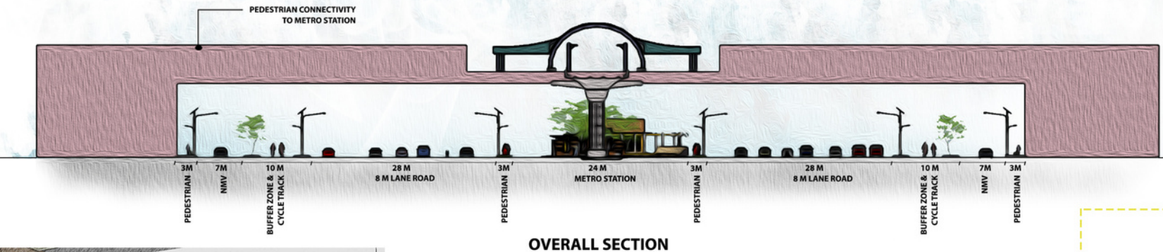
OVERALL SECTION
